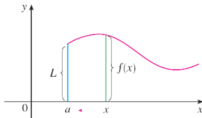
(b) \lim_{x \rightarrow a^+} f(x) = L
