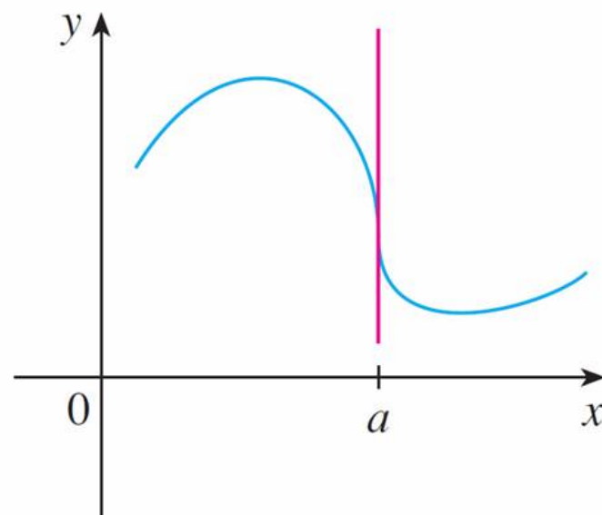
A vertical tangent
