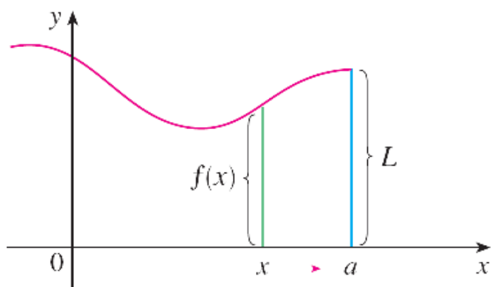
(a) \lim_{x \rightarrow a^-} f(x) = L
