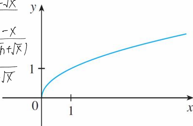
(a) f(x) = \sqrt{x}
