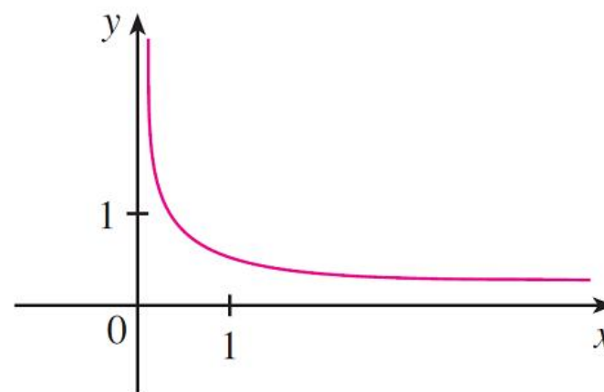
(b) f'(x) = \frac{1}{2\sqrt{x}}
