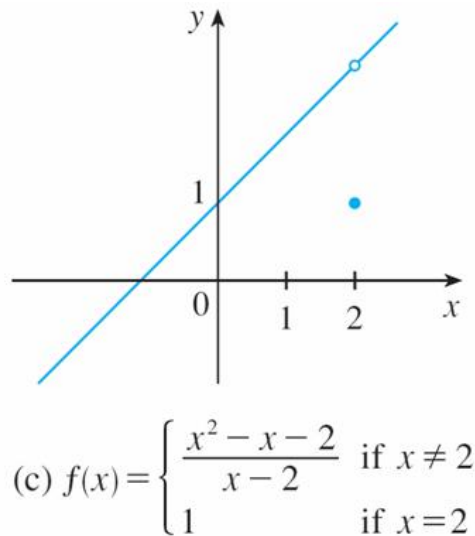
Graphs of the functions in Example 2
